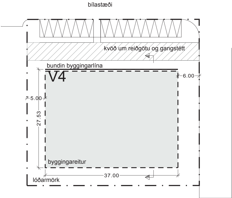
Grunnmynd, mkv.1:500
